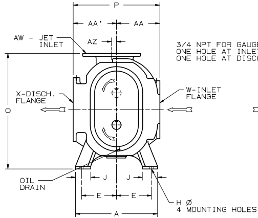
LEFT SIDE DISCHARGE FURNISHED WHEN SPECIFIED
