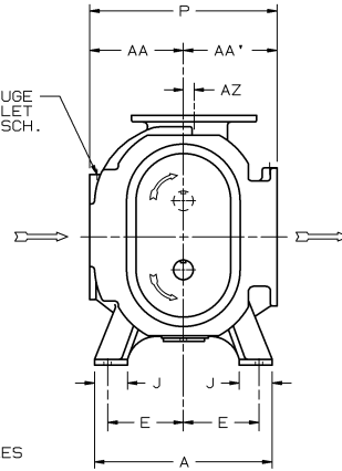
RIGHT SIDE DISCHARGE FURNISHED WHEN SPECIFIED
