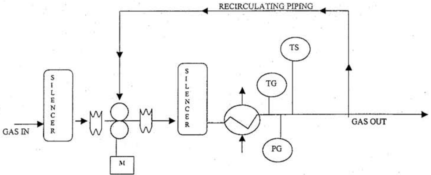
Typical DPJ Blower Layout
